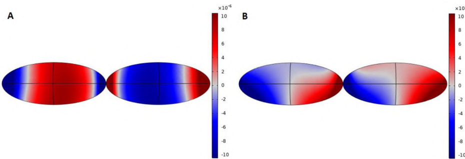
Fig. 5. Surface instant charge distribution for a NS ( 2a=1000 nm) at 1780 nm (A) for \varphi=0 and (B) for \varphi=2.25\pi where \varphi is phase of incident field. Red and blue colors represent charges of opposite signs. The areas in gray correspond to zero charge.
