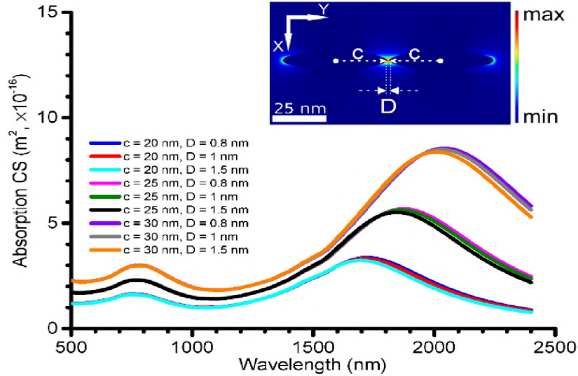
Fig.3 Simulated ACS of coupled MXene nanospheroids in end-to-end configuration with equal short semiaxes ( a = b = 5\text{nm} ) and varying long semiaxis ( c = 20, 25 or 30\text{ nm} ). Inset: electric field intensity map in the case of coupled spheroids with semiaxis c = 25\text{nm} and a = b = 5\text{nm} , irradiated by parallel electric field at 760 nm.
