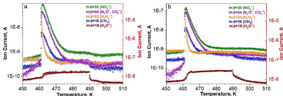
Fig. 7. Mass spectroscopy results for \text{Co}(\text{NO}_3)_2 + \frac{5}{10}\phi \text{C}_6\text{H}_{12}\text{N}_4 systems, when \phi = 0.75 (a) and \phi = 1.5 (b) heated at 30 \text{K} \cdot \text{min}^{-1} rate
