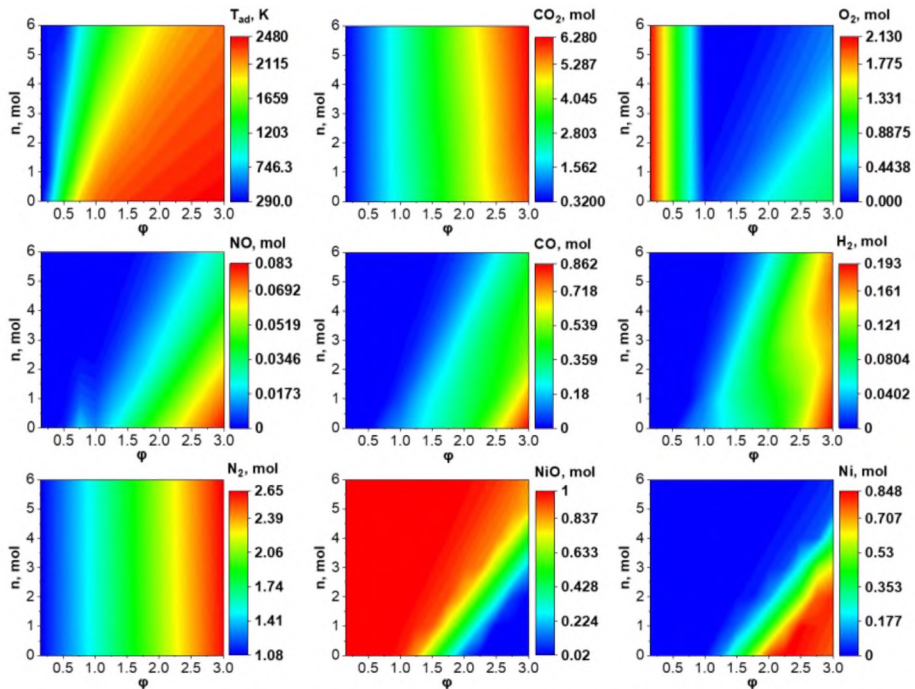
Fig. 1. Two-dimensional level plots for T_{ad} and equilibrium product for the Ni(NO_3)_2 + \frac{10}{9}\phi C_2H_5NO_2 + \frac{5}{2}(\phi - 1)O_2 + nH_2O system depend on \phi ratio and n (number of H_2O moles)
