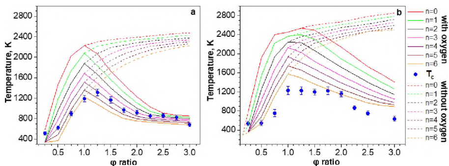
( T_c , blue data points) versus \phi ratio for the \text{Ni}(\text{NO}_3)_2 + \frac{10}{9}\phi \text{C}_2\text{H}_5\text{NO}_2 + \frac{5}{2}(\phi - 1) \text{O}_2 + n \text{H}_2\text{O} (a) and \text{Ni}(\text{NO}_3)_2 + \frac{5}{11}\phi \text{C}_6\text{H}_{12}\text{N}_4 + \frac{5}{2}(\phi - 1) \text{O}_2 + n \text{H}_2\text{O} (b) systems. Plots also include calculated T_{ad} values (solid and dashed lines)
