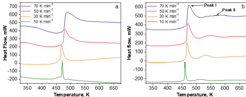
Fig. 6. DSC curves for \text{Co}(\text{NO}_3)_2 + \frac{5}{10}\phi \text{C}_6\text{H}_{12}\text{N}_4 systems, when \phi = 0.75 (a) and \phi = 1.5 (b) at different heating rates
