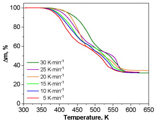
Fig.12. TGA analysis results of 3Ni(NO 3 ) 2 + Cu(NO 3 ) 2 + 5C 6 H 12 N 4 gel at 5, 10, 15, 20, 25, 30 K/s heating rates
