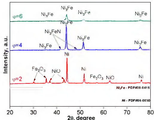
Fig. 9. X-ray diffraction patterns of the combustion products of the 3\text{Ni}(\text{NO}_3)_2 \cdot 6\text{H}_2\text{O}\text{-}\varphi\text{Fe}(\text{NO}_3)_3 \cdot 9\text{H}_2\text{O}\text{-}\varphi\text{C}_6\text{H}_{12}\text{N}_4 system for different values of \varphi
